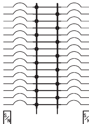
400 A or 600 A PowerPacT L-Frame Main Circuit Breaker with Sub-feed Circuit Breaker
