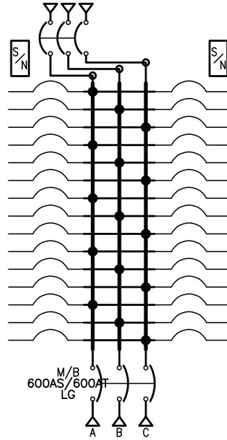
400 A or 600 A PowerPacT L-Frame Main Circuit Breaker with Sub-feed Circuit Breaker
