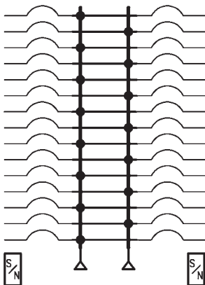
400 A or 600 A PowerPacT L-Frame Main Circuit Breaker with Feed-Thru Lugs
