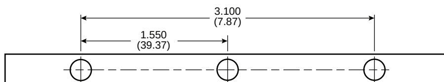
Figure 1 - Distance Between Mounting Holes (in Ground Bar Kits) —In (mm)
