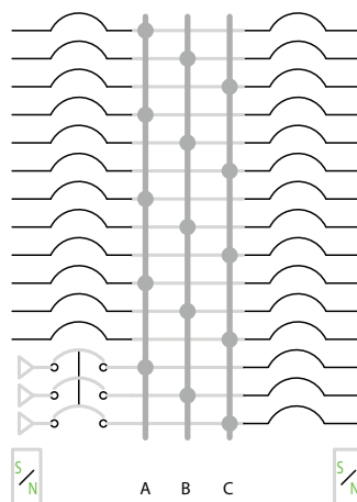
125 A Max. Branch Mounted Main Circuit Breaker
