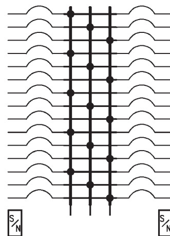
15–250 A Main Circuit Breaker Types H-, or J-Frame
