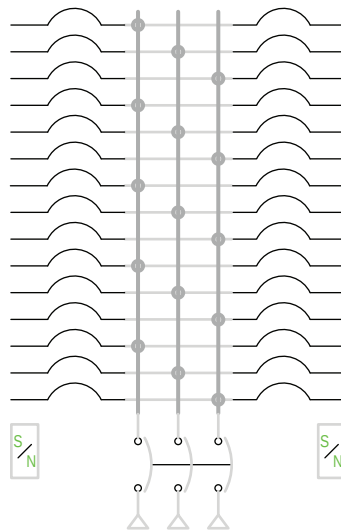
800 A Max. Main Circuit Breaker (M- or P-Frame)
