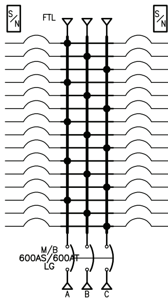
400 A or 600 A PowerPacT L-Frame Main Circuit Breaker with Feed-Thru Lugs
