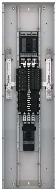
800 A MG Main Breaker Panelboard
