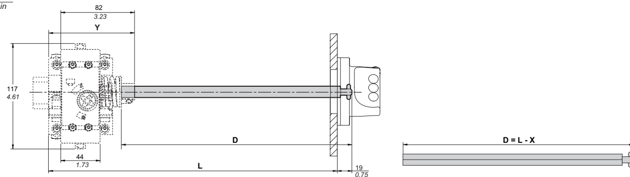
Rotary handle: side mounted control
