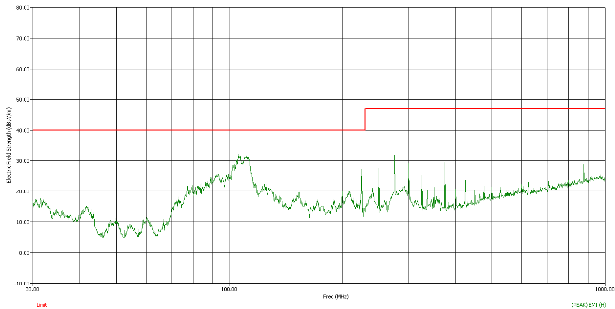
Figure 8: Graphical representation of Radiated emission (on line mode)
