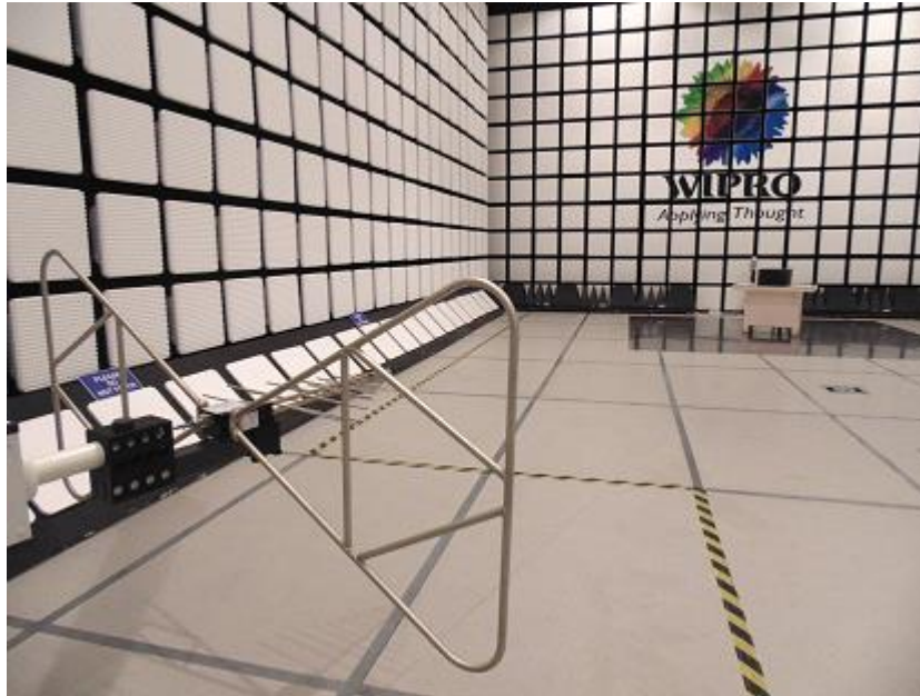
Figure 7: Photo of Radiated emission test setup
