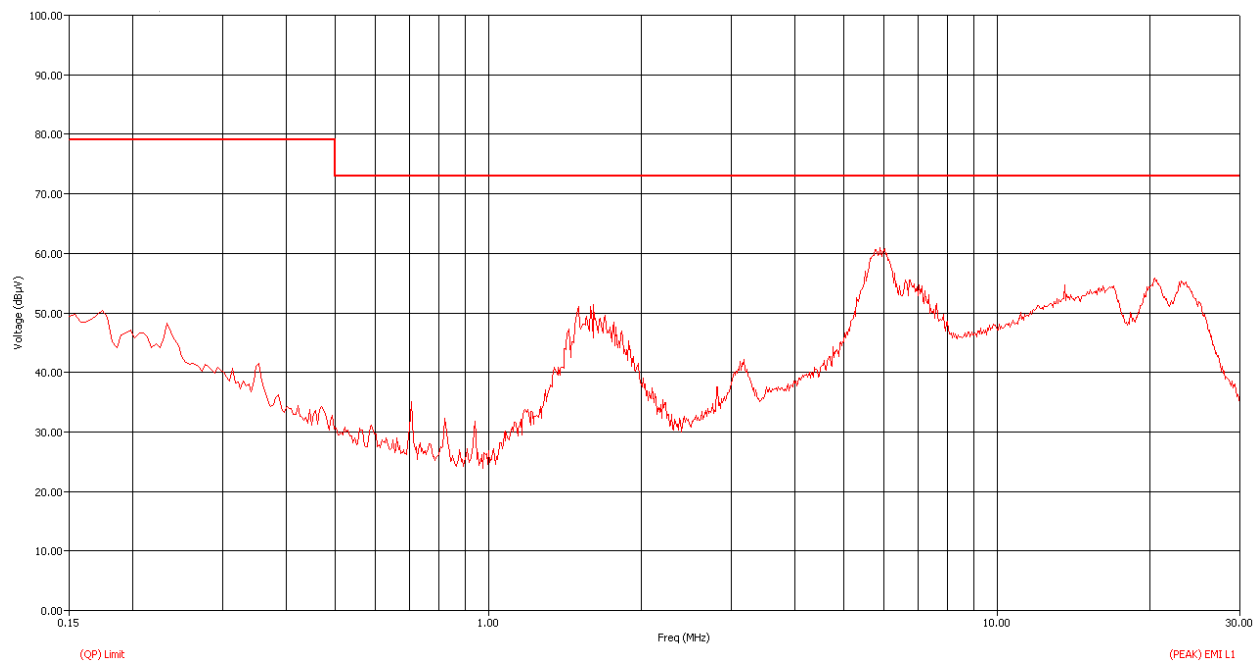
Figure 2 : Graphical representation of conducted emissions (on line mode)
