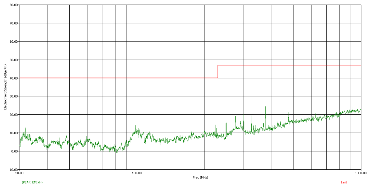
Figure 9: Graphical representation of Radiated emission (on battery mode)
