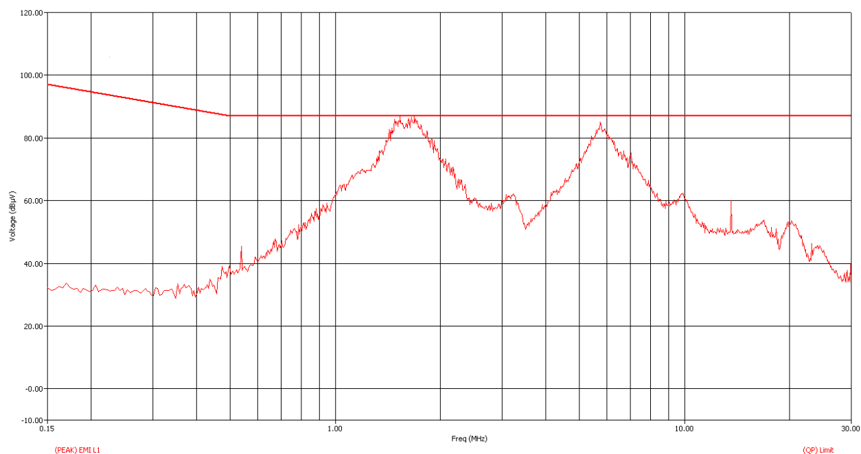
Voltage – Peak Measurement
