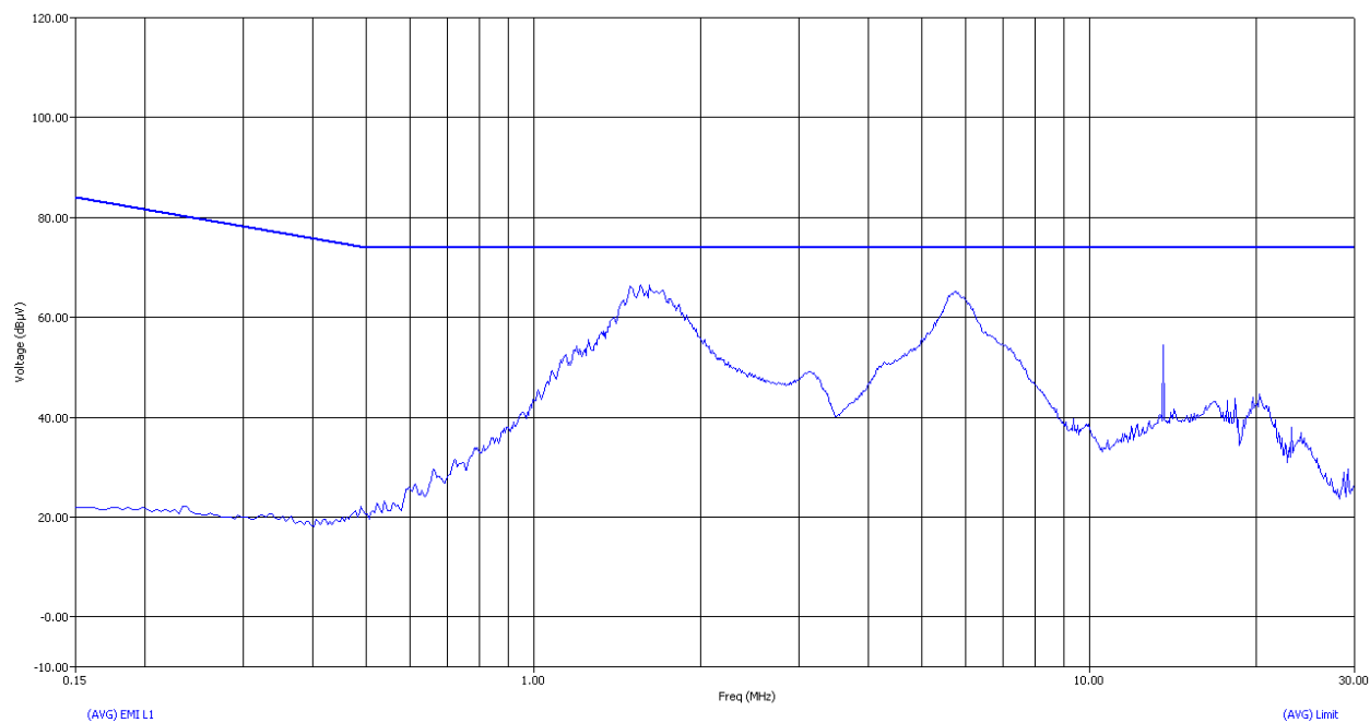
Voltage – Average Measurement
