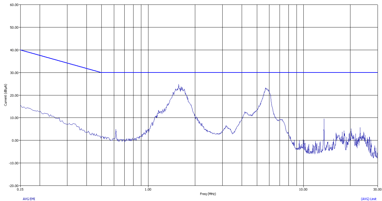
Current – Average Measurement
