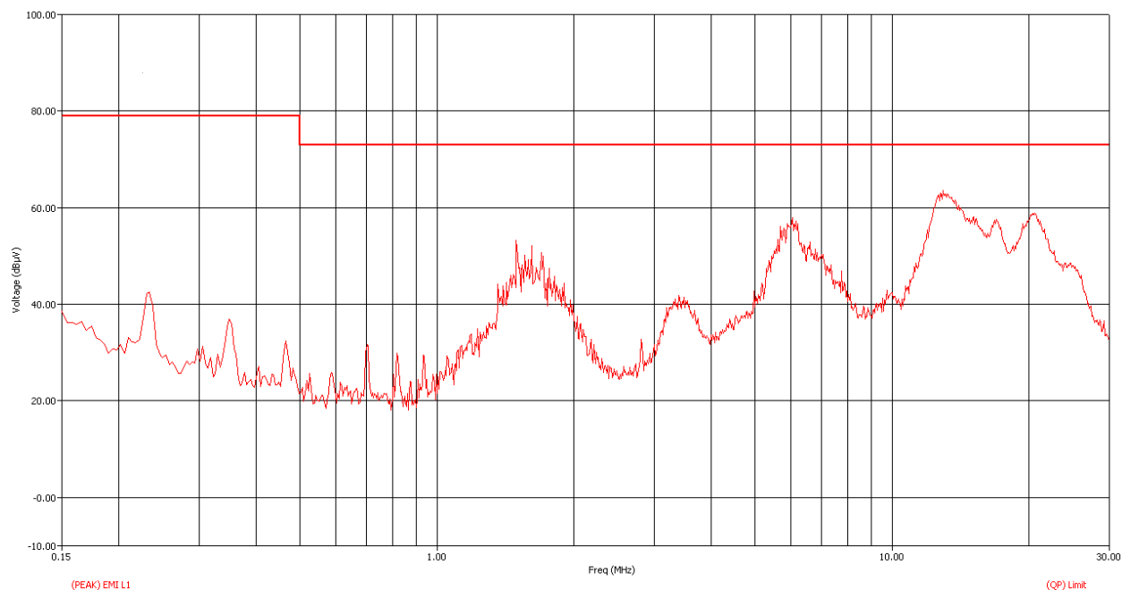
Figure 3: Graphical representation of conducted emissions (on battery mode)
