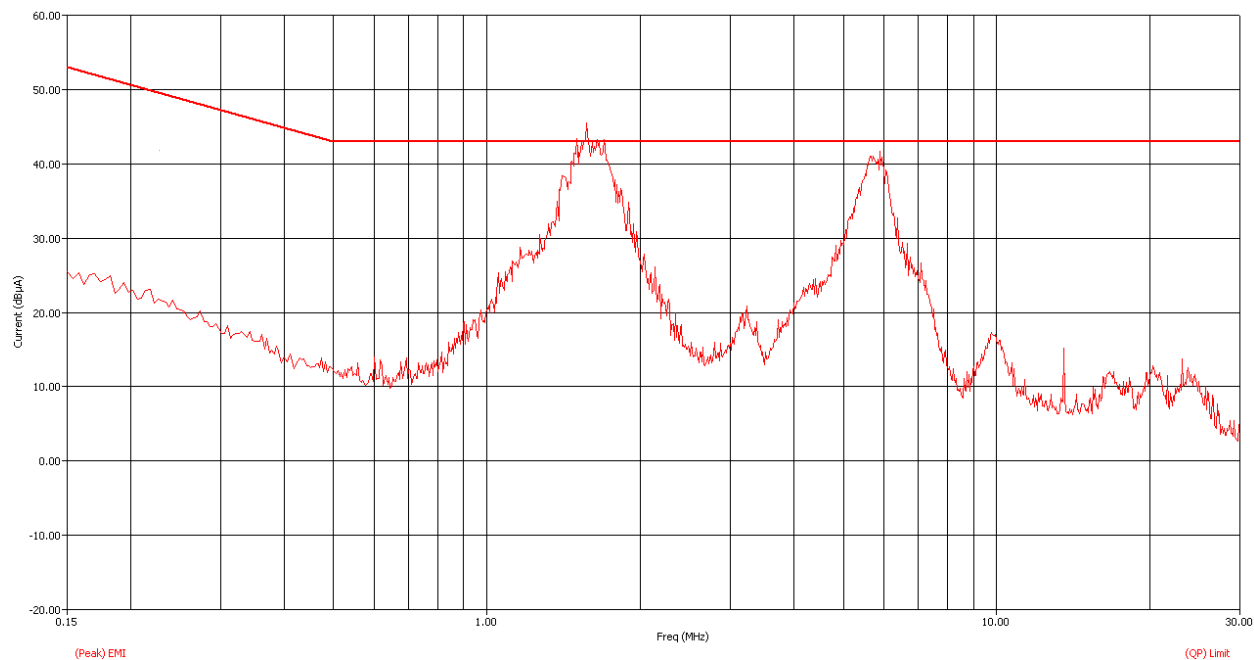
Current – Peak Measurement
