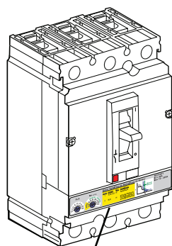
J-Frame Motor Circuit Protector JL36250M75
