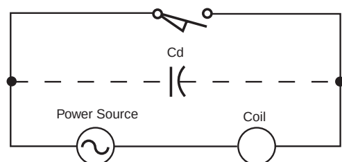
Figure 1: Control Device
