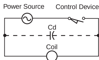
Figure 2: Power Source
