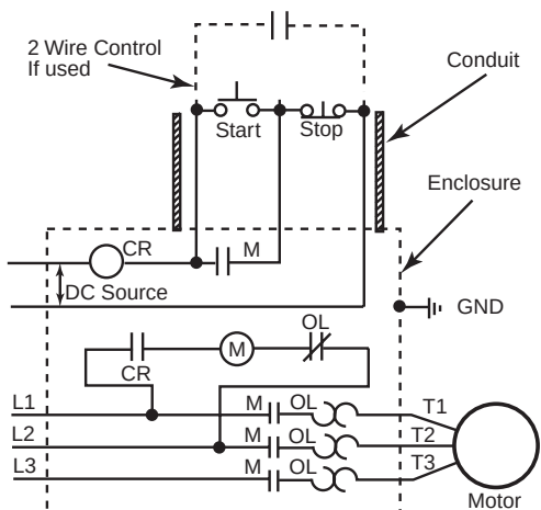
Figure 7: Interposing DC Control Relay
