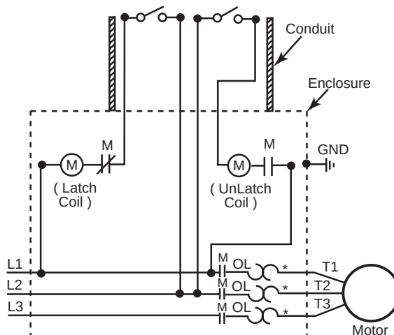
Figure 8: Mechanically Held Contactor or Relay
