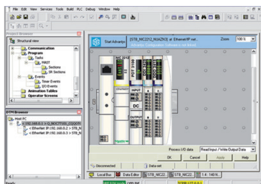
DTM editor (Modicon STB island)
