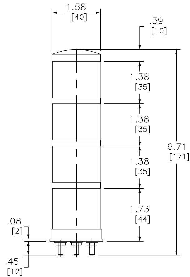
FRONT
