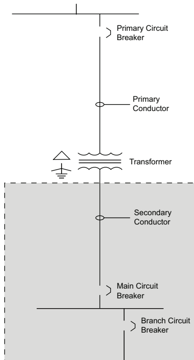
Figure 1: Transformer Through-Fault Protection Zone
