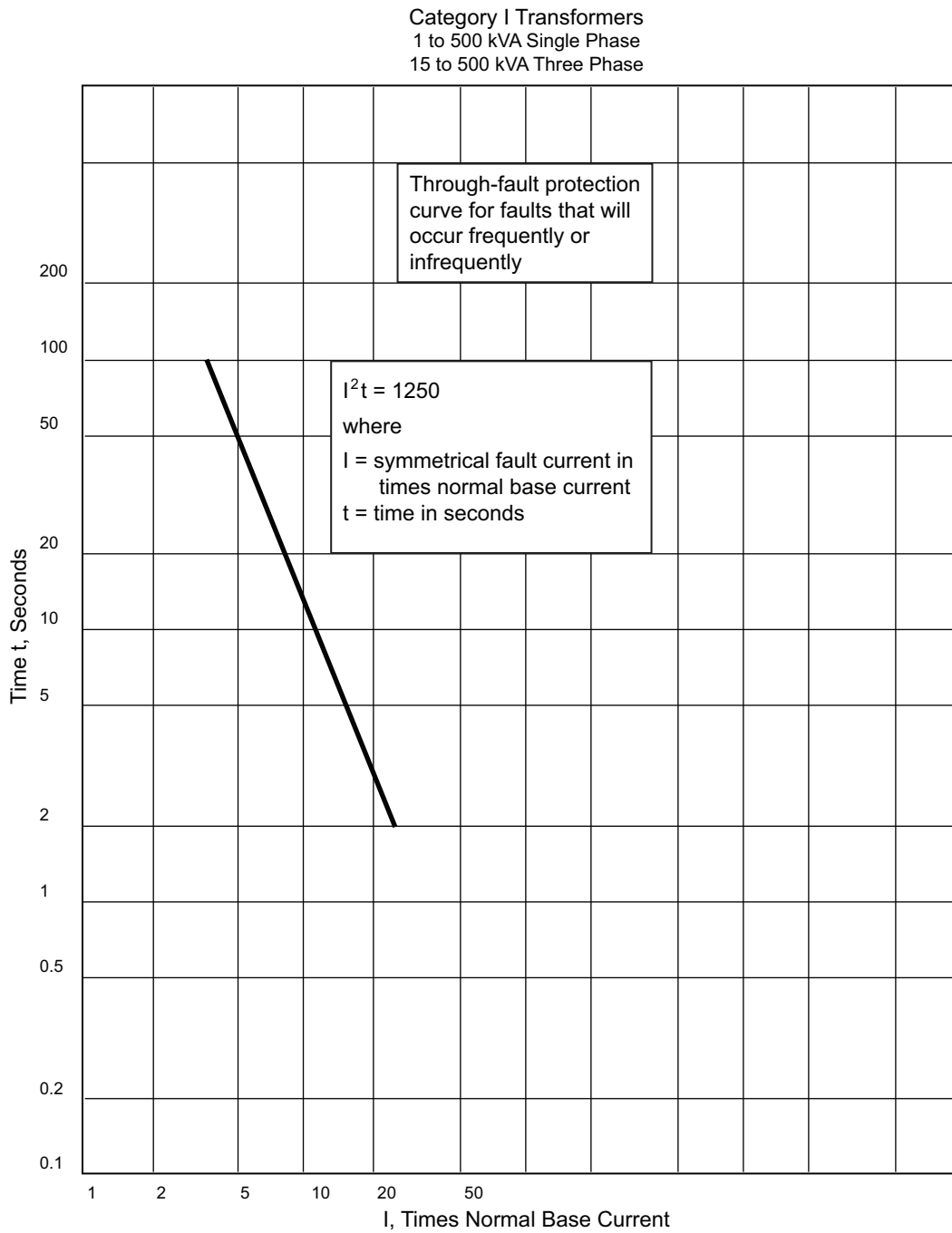
Figure 2: Category I Transformers Through-Fault Curve
