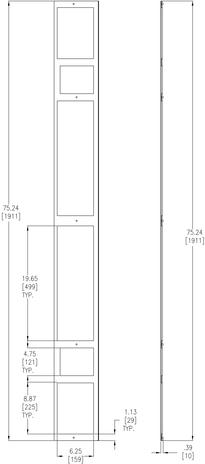
FRONT VIEW
