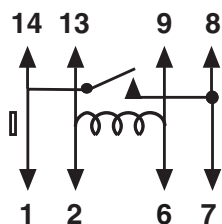
Figure E SPST-NO Without diode
