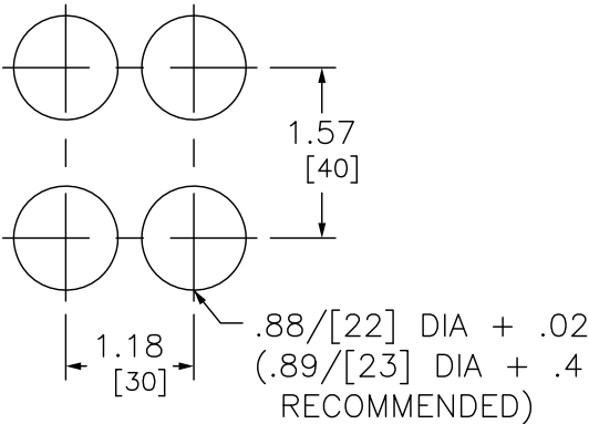
PANEL CUT-OUTS FOR INSTALLATION
