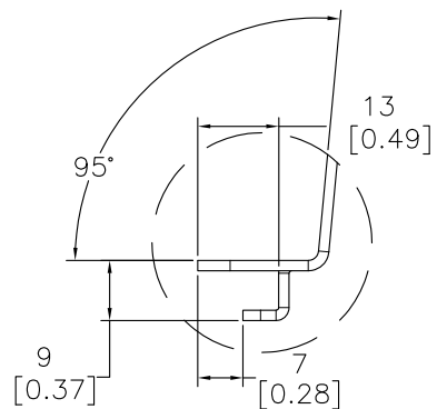
DETAIL-A (ENLARGED)
