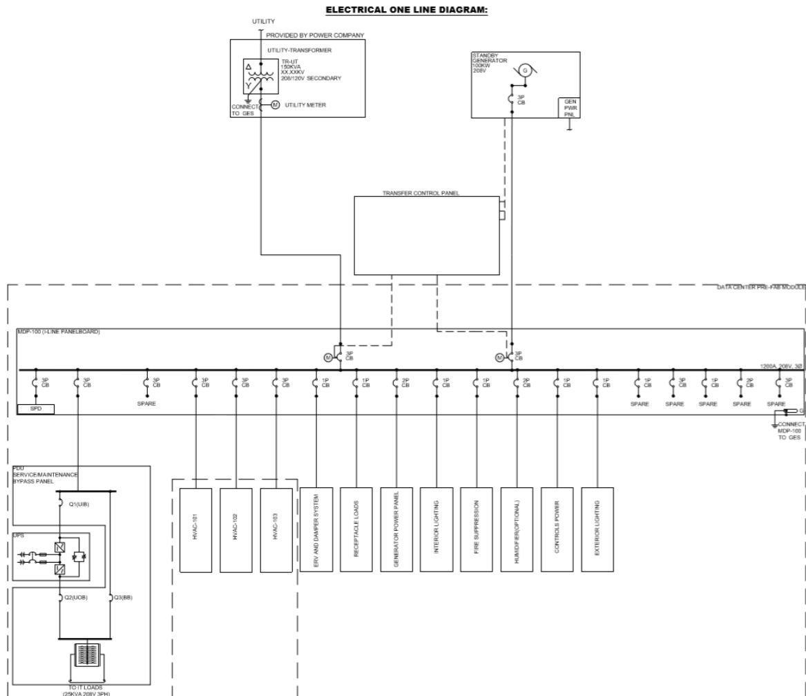
Proposed Electrical Single-Line Drawing E400
