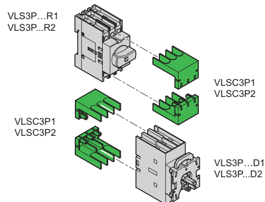
Figure 4: Terminal covers
