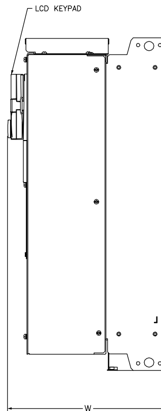
RIGHT VIEW
