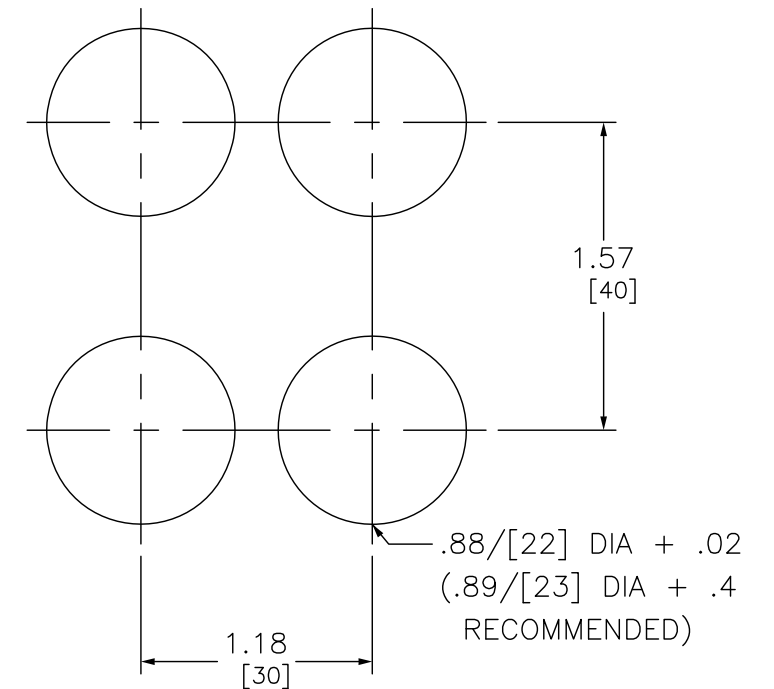
PANEL CUT-OUTS FOR INSTALLATION
