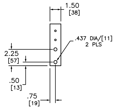
H TERMINAL DETAIL
