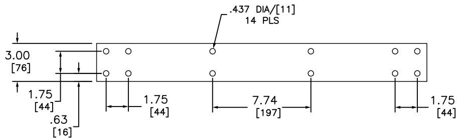
X TERMINAL DETAIL
