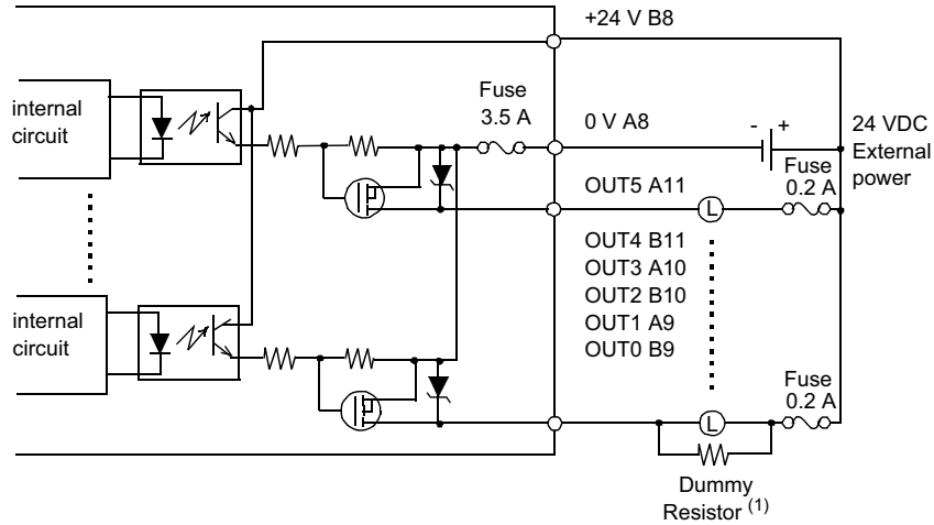
XBT GC1100U Output Circuit (Sink type):
