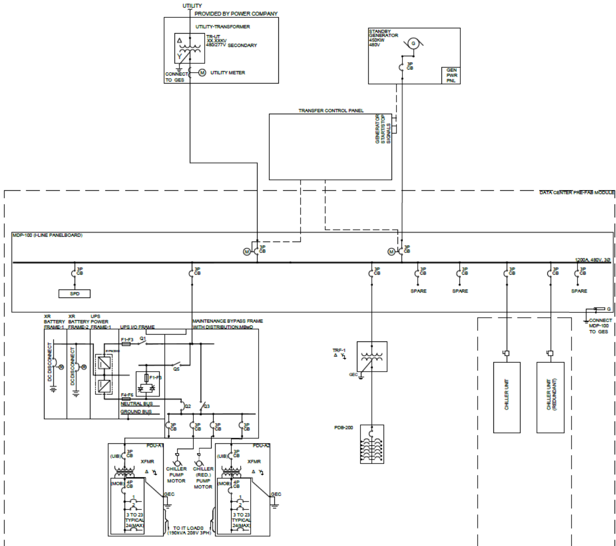
Proposed Electrical Single-Line Drawing E400
