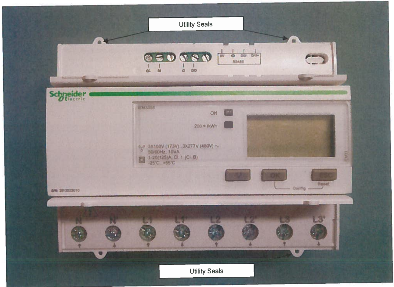
Photograph of Meter and Sealing Plan for iEM33xx
