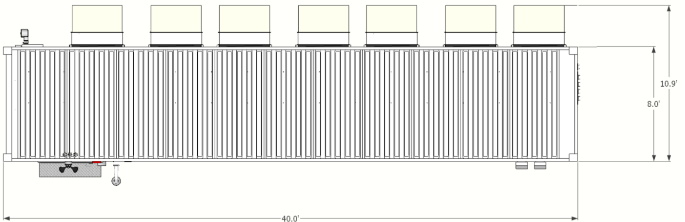
Exterior View with Dimensions
