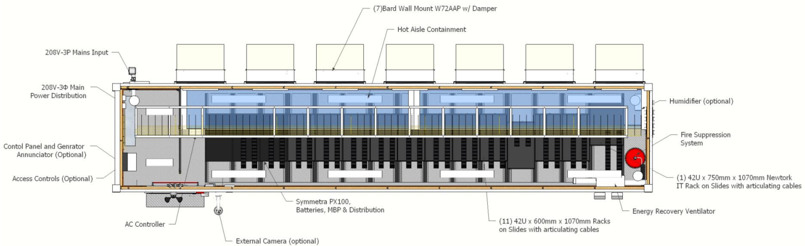
Interior Overhead View
