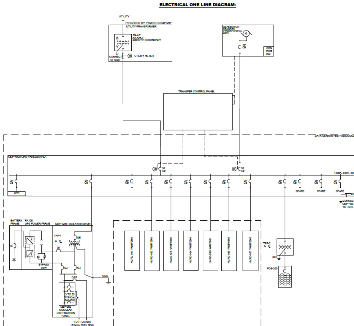
Proposed Electrical Single-Line Drawing E400
