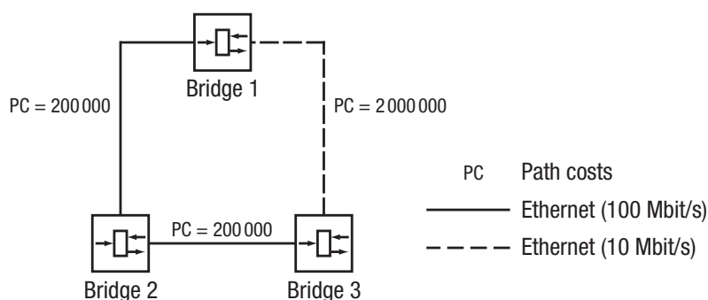
Figure 9: Path costs
