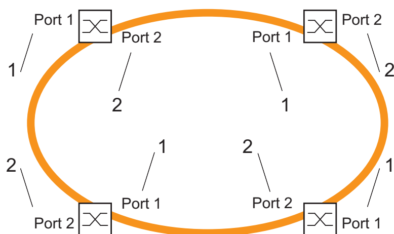
Figure 7: Example for a HIPER-Ring with straight cables
