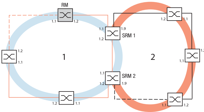
Figure 16: Example for Sub-Ring structure 1 blue ring = Base Ring 2 orange ring = Sub Ring SRM = Sub-Ring Manager RM = Ring Manager
