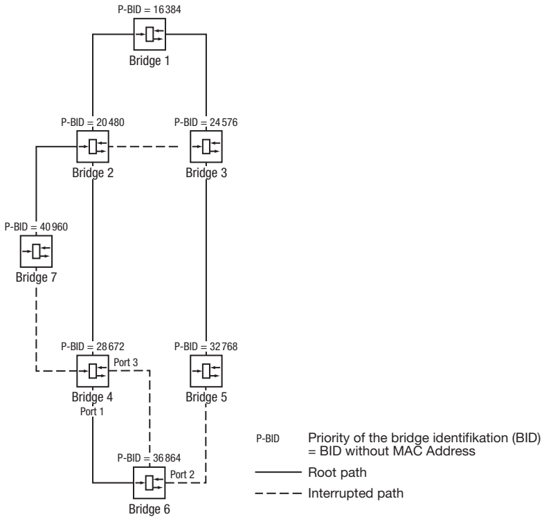
Figure 44: Example of root path determination
