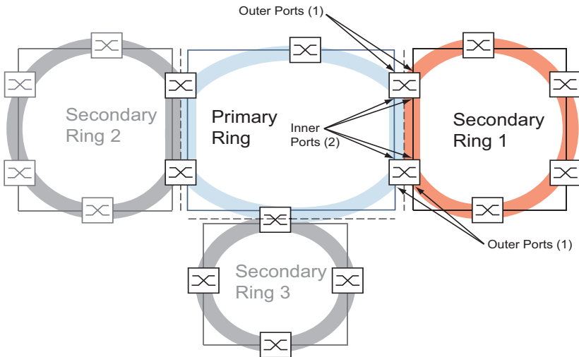
Figure 54: Primary ring with 3 secondary rings connected via Dual RSTP, 1: outer ports 2: inner ports
