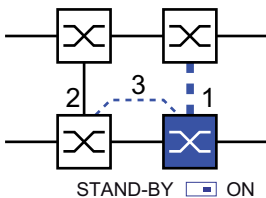
Figure 36: Two-Switch coupling with control line
