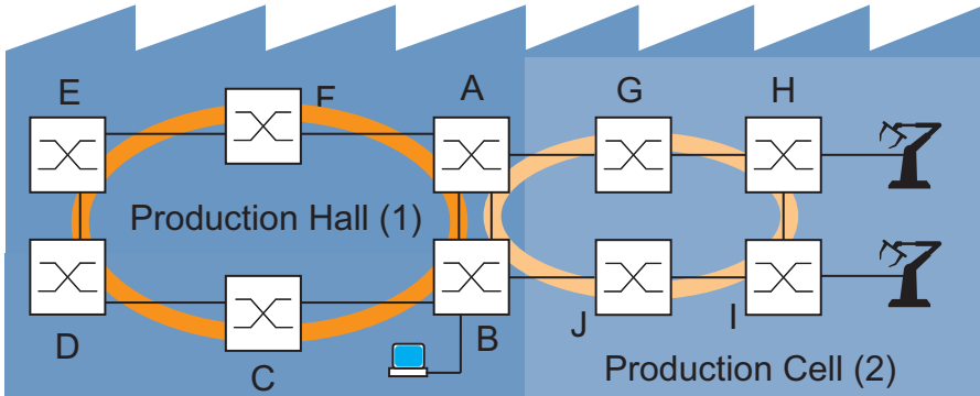
Figure 59: Example of a production cell in a production hall, topology when using Dual RSTP 1: production hall 2: production cell
