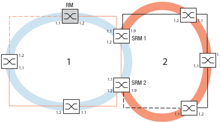
Figure 12: Example for Sub-Ring structure
