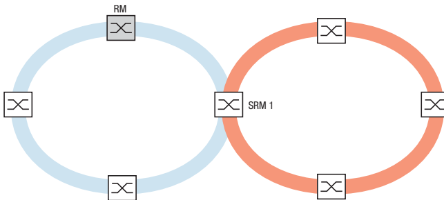
Figure 15: Special case: a Sub-Ring Manager manages both ends of a Sub-Ring at different ports (Single Sub-Ring Manager).
