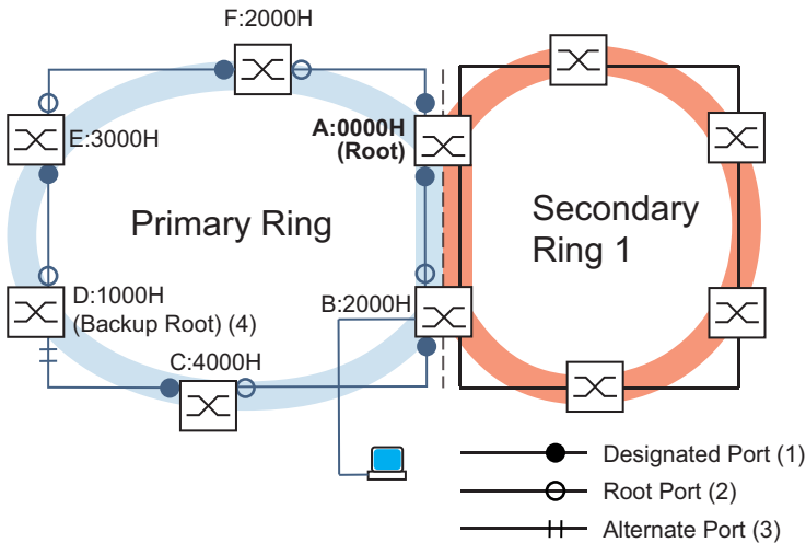
Figure 55: Primary ring with 1 connected secondary ring, with details for the primary ring, A..F: bridge identifiers 0000H..4000H: bridge priorities in the primary ring 1: designated port 2: root port 3: alternate port 4: backup root bridge for primary ring
