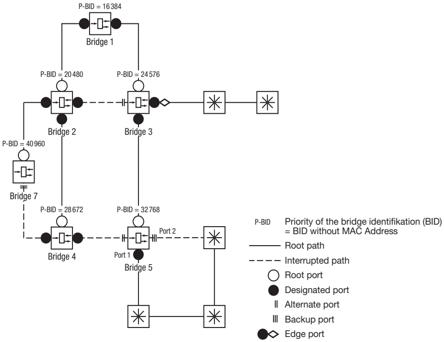
Figure 47: Port role assignment
