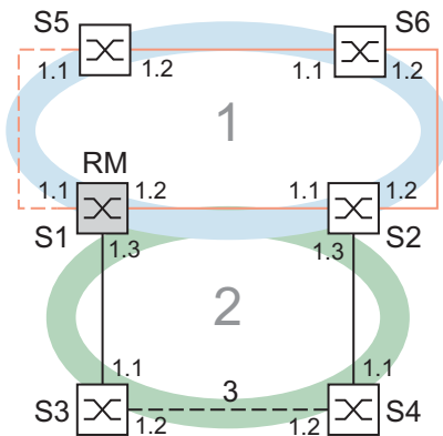
Figure 53: Application example for the combination of RSTP and MRP 1: MRP-Ring, 2: RSTP-Ring, 3: Redundant RSTP connection RM: Ring Manager S2 is RSTP Root Bridge S1 is RSTP Backup Root Bridge
