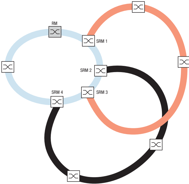
Figure 13: Example of an overlapping Sub-Ring structure
