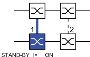
Figure 27: Two-Switch coupling 1: Coupling port 2: Partner coupling port
