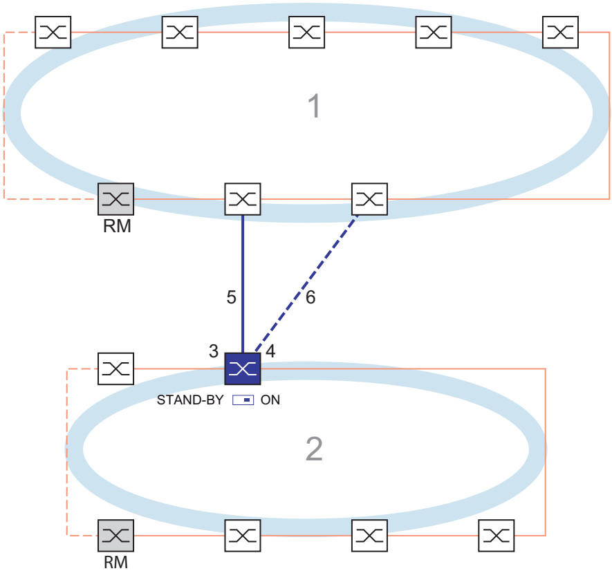
Figure 20: Example of one-Switch coupling
