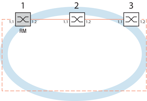
Figure 9: Example of Fast HIPER-Ring RM = Ring Manager — main line - - - redundant line
