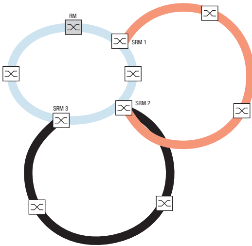
Figure 14: Special case: a Sub-Ring Manager manages 2 Sub-Rings (2 instances). Depending on the device type, you can configure additional instances.
