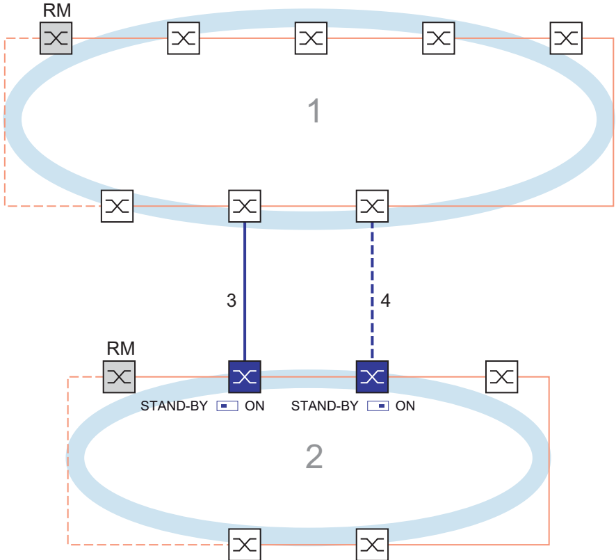
Figure 26: Example of two-Switch coupling
