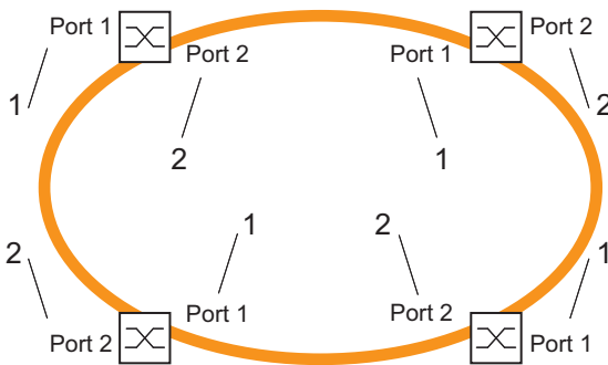
Figure 11: Example for a HIPER-Ring with straight cables 1 = Manual Cable Crossing disabled 2 = Manual Cable Crossing enabled
