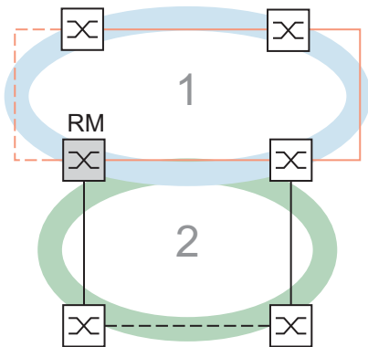
Figure 52: Combination of RSTP and MRP
