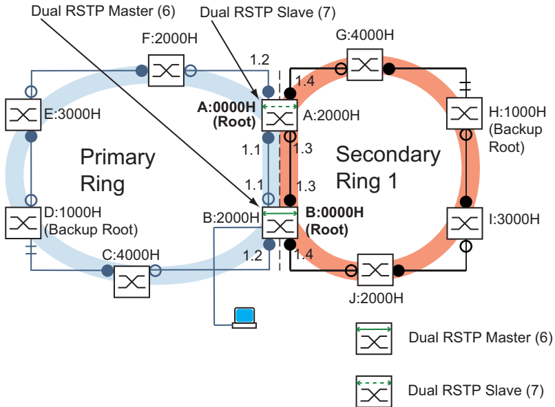
Figure 60: Schematic representation of Dual RSTP network topology, 6: Dual RSTP master 7: Dual RSTP slave
