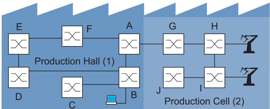
Figure 58: Example of a production cell in a production hall, topology before using Dual RSTP 1: production hall 2: production cell
