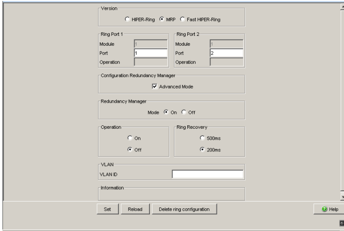
Figure 8: Ring Redundancy dialog (TCSESM-E)
