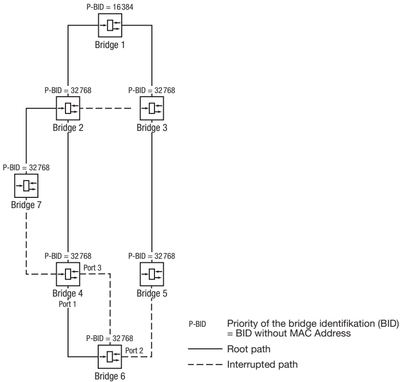
Figure 45: Example of root path manipulation
