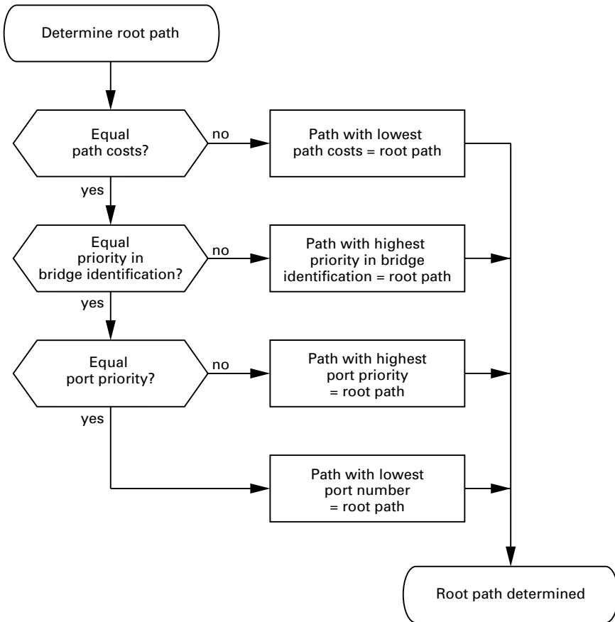
Figure 43: Flow diagram for specifying the root path
