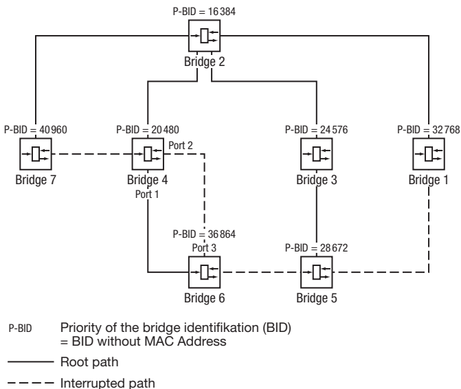
Figure 46: Example of tree structure manipulation
