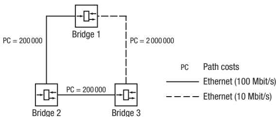
Figure 41: Path costs
