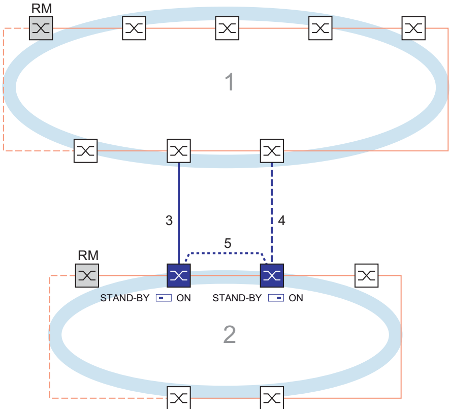
Figure 33: Example of Two-Switch coupling with control line
