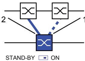
Figure 21: One-Switch-coupling 1: Coupling port 2: Partner coupling port
