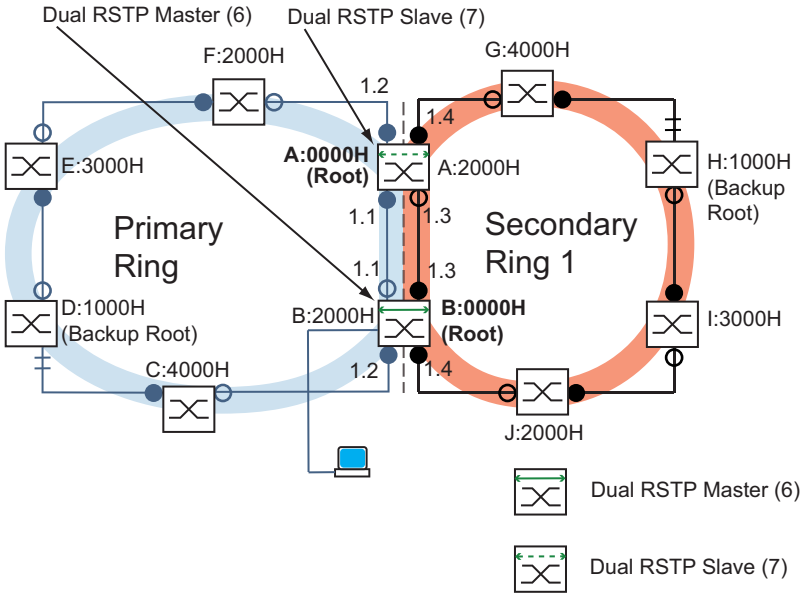
Figure 57: Primary ring with 1 connected secondary ring, with port numbers and Dual RSTP coupling roles, 6: Dual RSTP master 7: Dual RSTP slave
