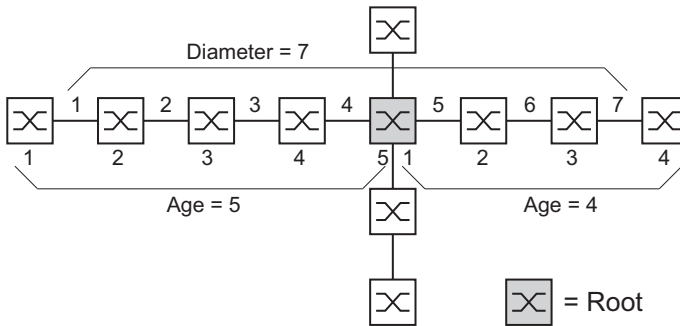
Figure 50: Definition of diameter and age
