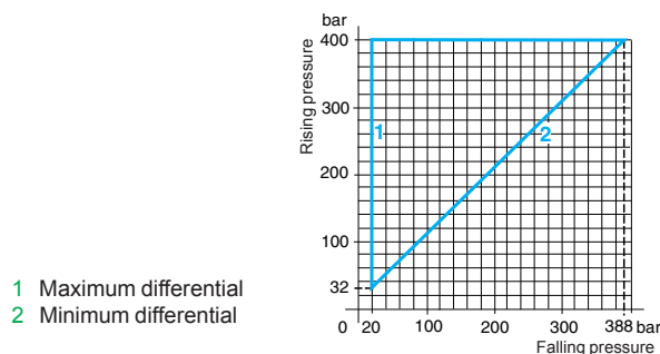
XMLG400●●1TQ
