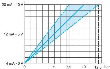
Analog output curve
