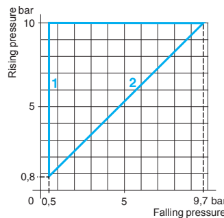
Pressure sensor operating curves
