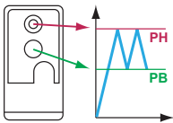
Adjustable differential
