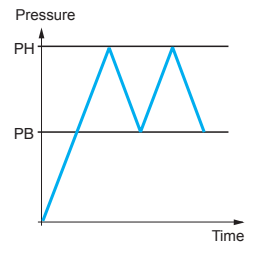
1 Maximum differential 2 Minimum differential — Adjustable value
