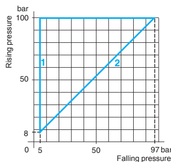
XMLG100●●1TQ
