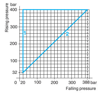
1 Maximum differential 2 Minimum differential — Adjustable value
