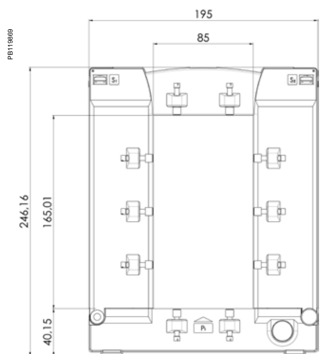
GJ Dimensions
