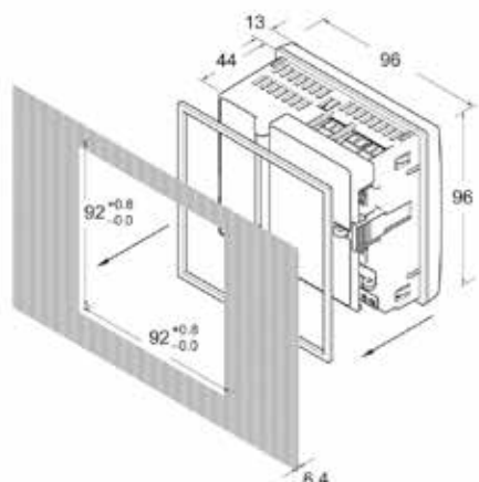
Dimensions PM5350IB
