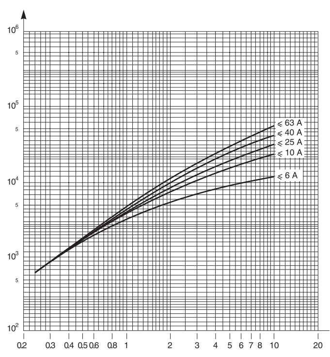
Figure 99: UL 1077 Recognized C60 2P, 3P, and 4P (480Y/277 Vac) Maximum Let-Through I²t Current
