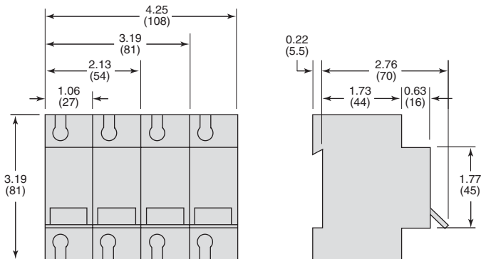
Figure 49: C120 IEC Circuit Breaker
