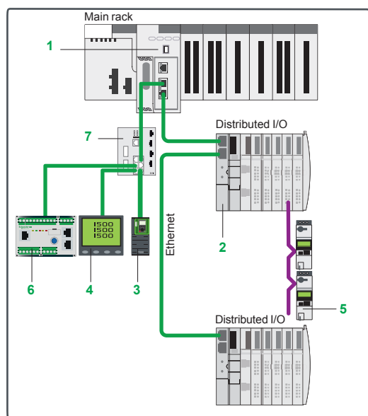
Distributed I/O architecture: devices distributed over Ethernet with DRS
