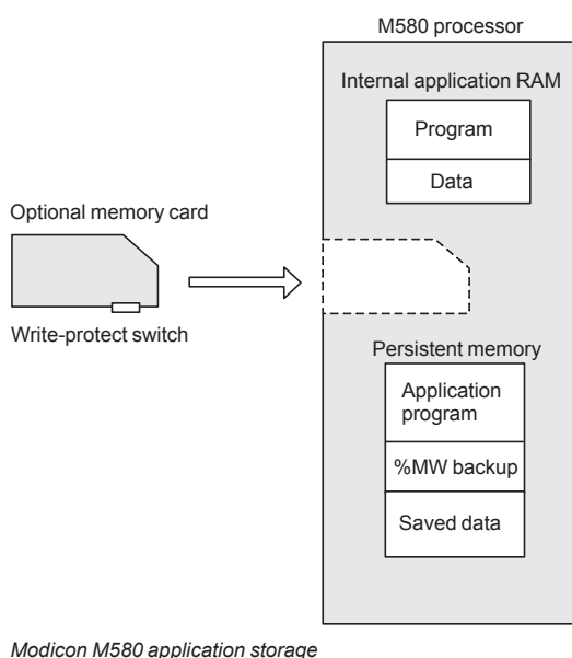
Modicon M580 application storage
