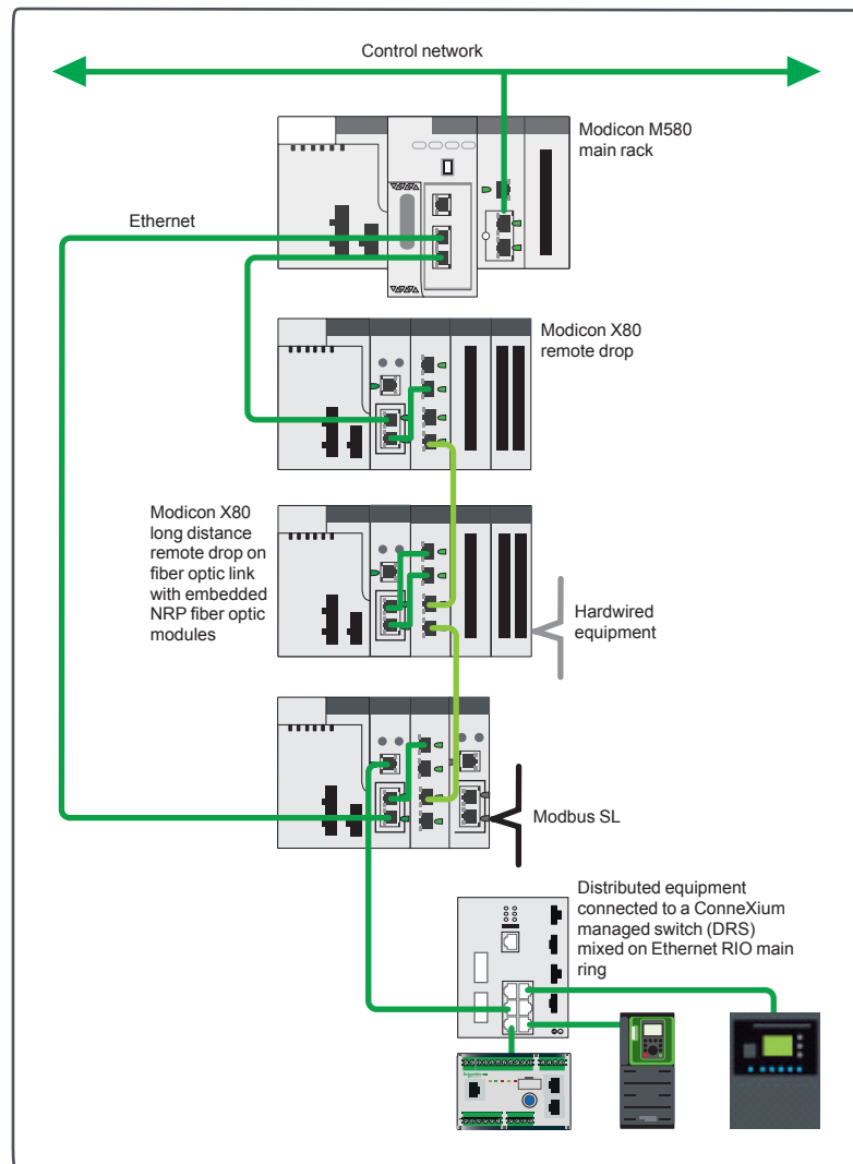
Example of a standalone architecture: Hydropower application
