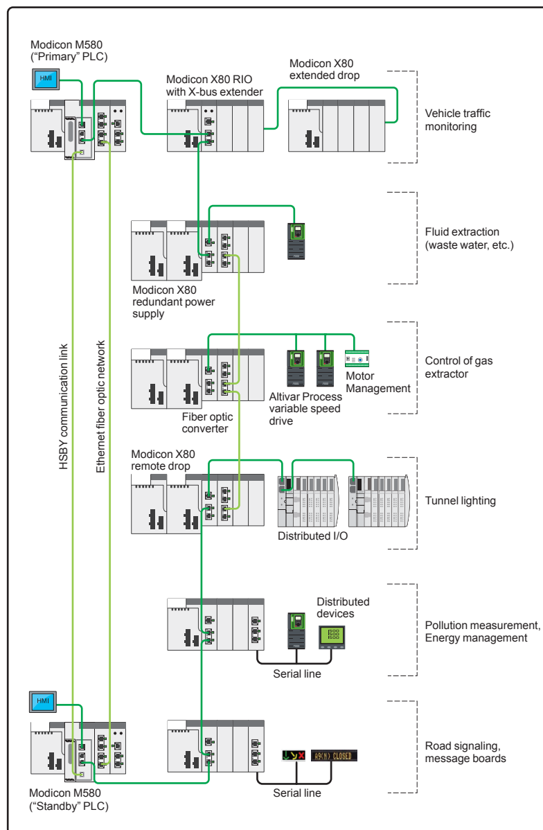
Example of a high-availability architecture: Tunnel application
