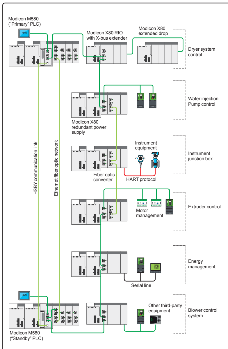
Example of a high-availability architecture: Petrochemical application
