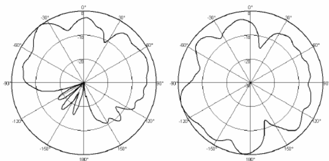
E-Plane Pattern
