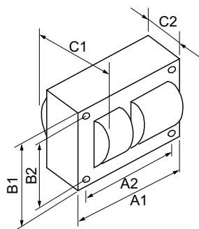
MH BAL 350W M131 QUAD KIT
