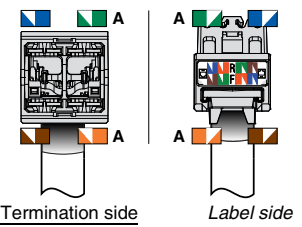
Termination side
