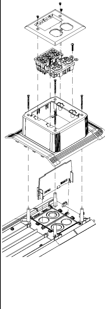
POWER/DATA APPLICATION
