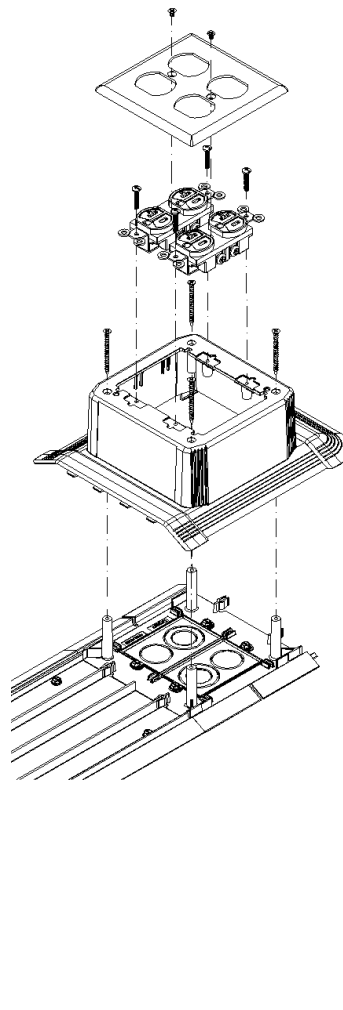
POWER APPLICATION
