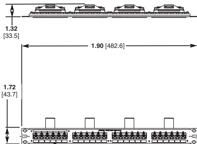
24-Port
