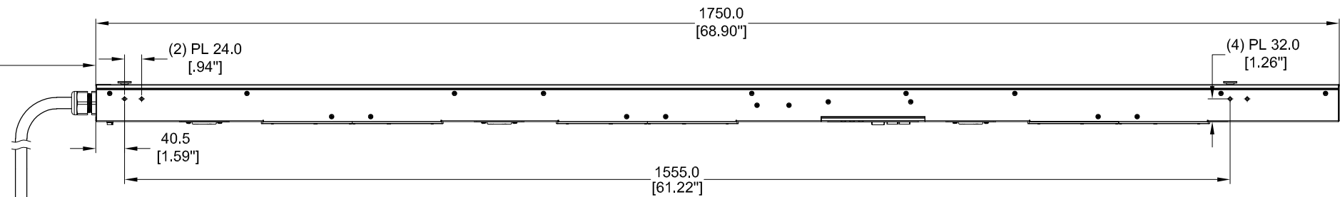
RIGHT VIEW
