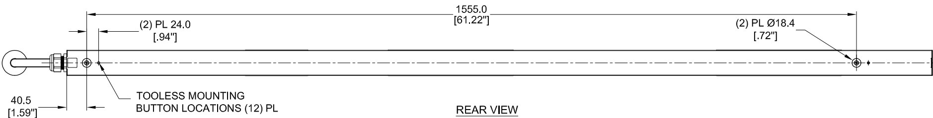
REAR VIEW
