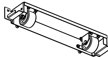
FIXED CASTER AND BRACKET ASSEMBLY
