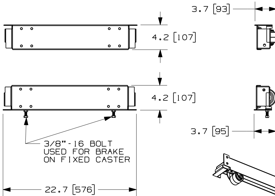
SWIVEL CASTER AND BRACKET ASSEMBLY
