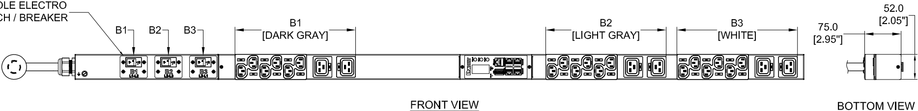
BOTTOM VIEW
