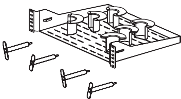
PZCHSM2 PANZONE Horizontal Slack Manager
