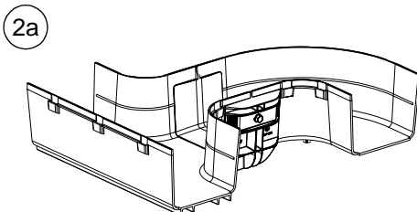
Fitting-to-Fitting Application
