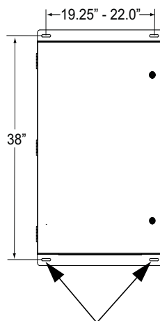
Hole Locations for Wall Mounting
