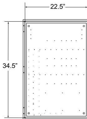
Dimensions for Wall Mounting without Flanges
