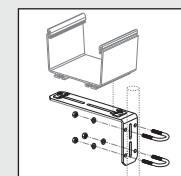
FR6USB – Underfloor Pedestal QuikLock™ Bracket (page J.33)
