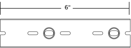
Minimum mounting rivet distance for ducts 1.5" wide.
