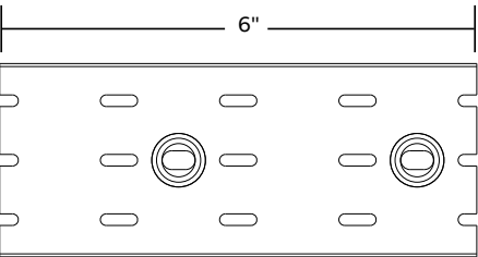
Minimum mounting rivet distance for ducts greater than 1.5" wide. Installed top and bottom.
