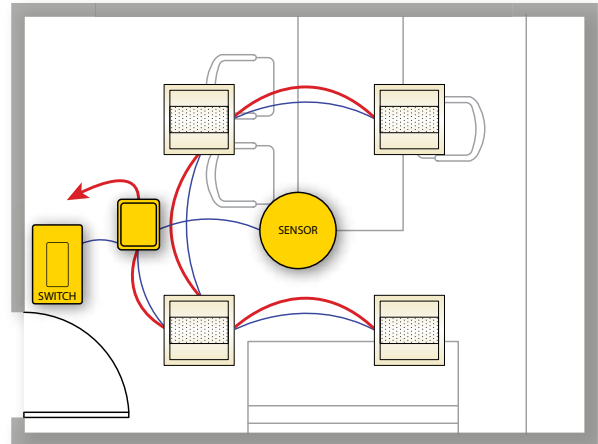
— Line-voltage wiring — Low-voltage wiring
