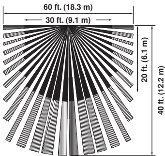
Figure 1 - Field-of-View (Horizontal)
