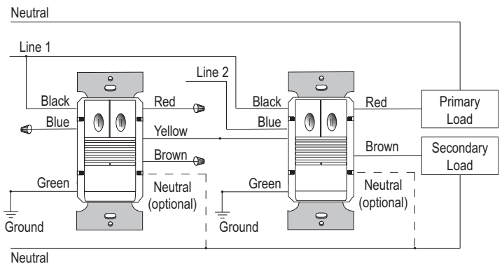
Two-phase Wiring
