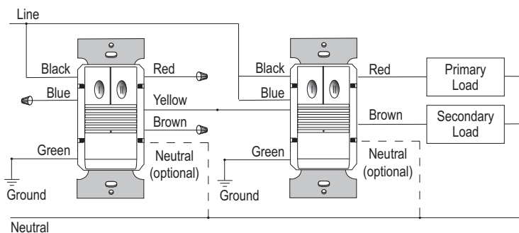
Bi-level Wiring (PW-302-347 up to 4 sensors)
