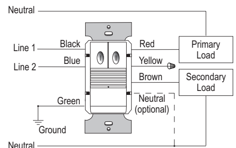
PW-302-347 Dual Circuit Wiring
