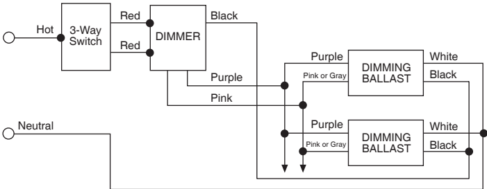
Figure 2 – 3-Way Wiring
