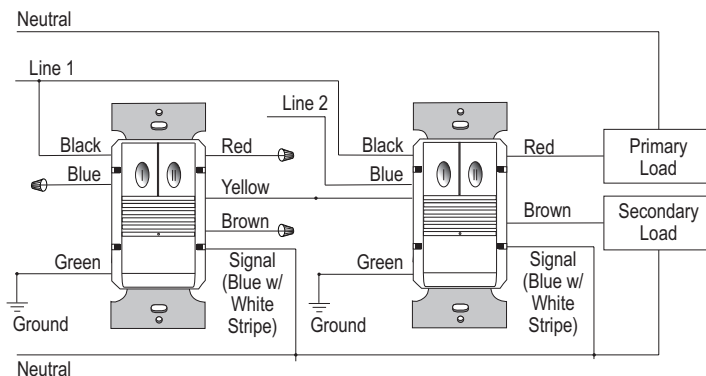
Two-phase Wiring
