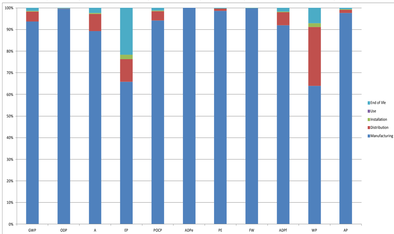
% ENVIRONMENTAL IMPACT PER LIFE CYCLE STAGE OF REFERENCE PRODUCT
