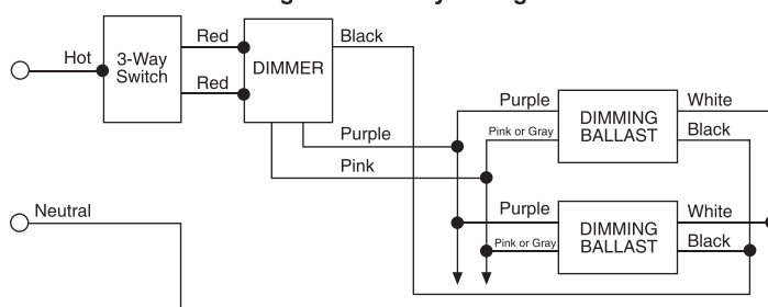
Figure 2 – 3-Way Wiring
