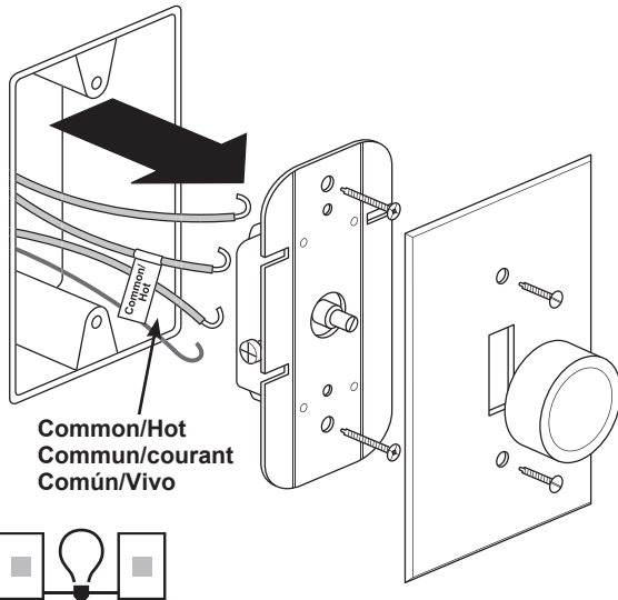
3-Way In a 3-Way circuit, identify the Common/ Hot wire — connected to the terminal marked Common or the odd-colored terminal screw.
