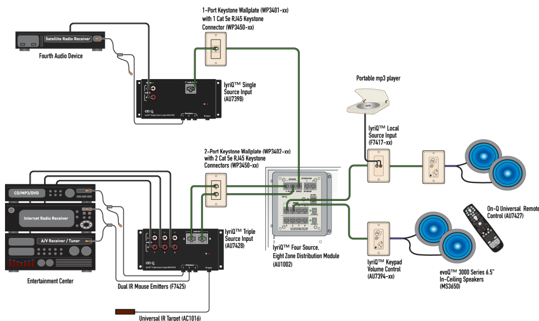
Optional components and Category 5 wiring to control four audio devices
